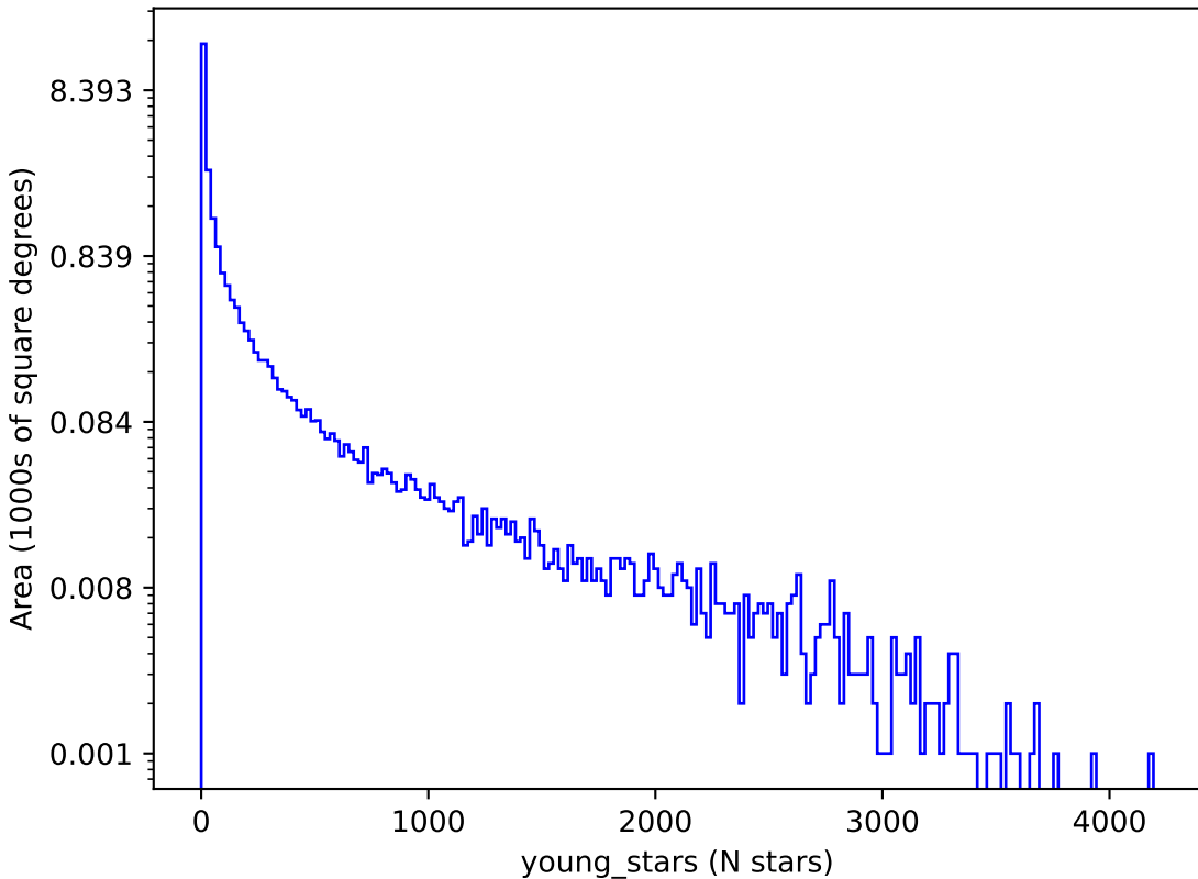
too_elab_r8_d3_gz_v3.4_10yrs : young_stars
