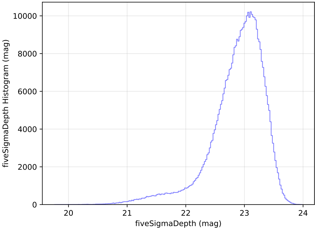
too_elab_r8_d3_gz_v3.4_10yrs z: fiveSigmaDepth Histogram
