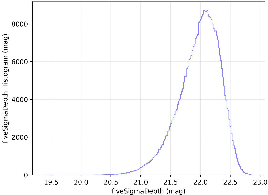
too_elab_r8_d3_gz_v3.4_10yrs y: fiveSigmaDepth Histogram
