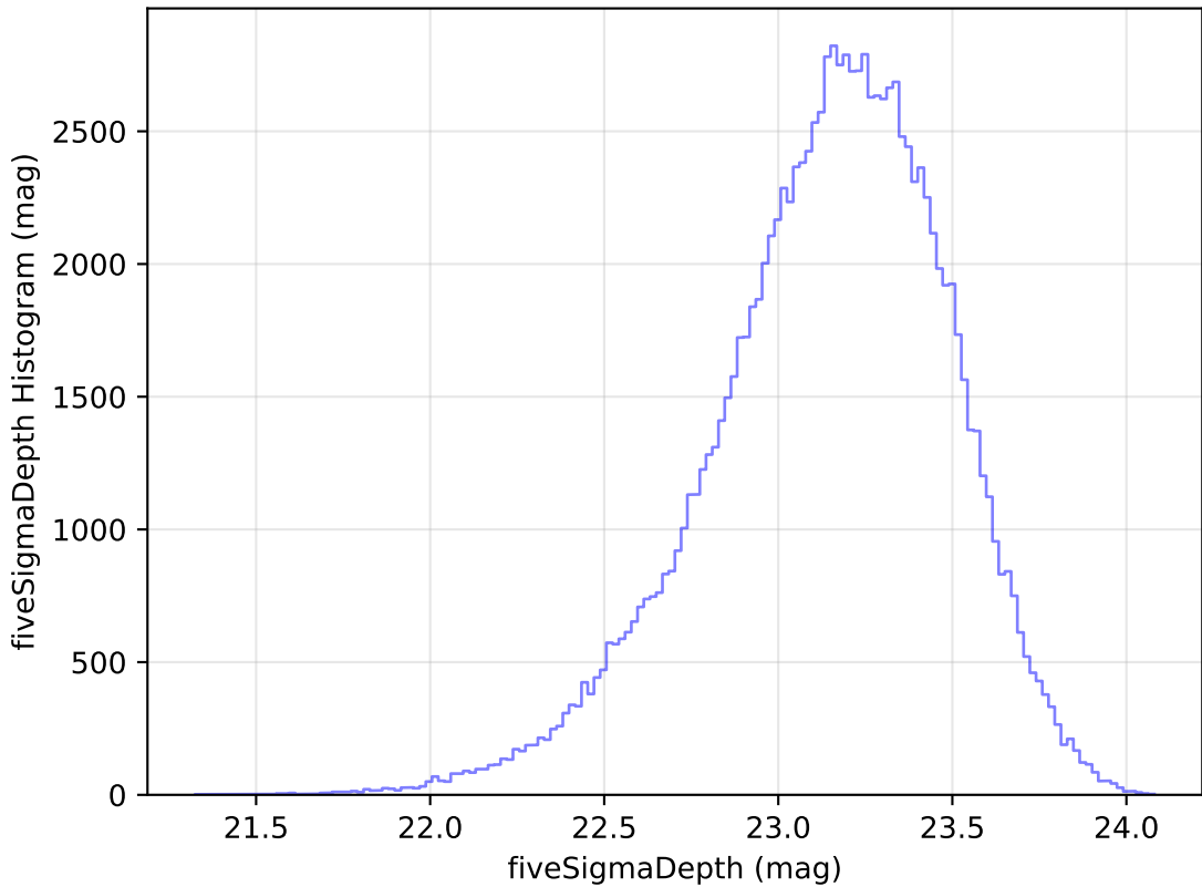
too_elab_r8_d3_gz_v3.4_10yrs u: fiveSigmaDepth Histogram
