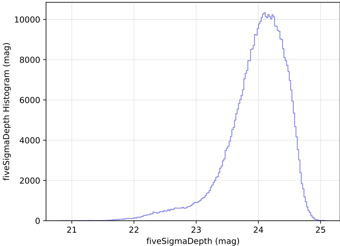
too_elab_r8_d3_gz_v3.4_10yrs r: fiveSigmaDepth Histogram
