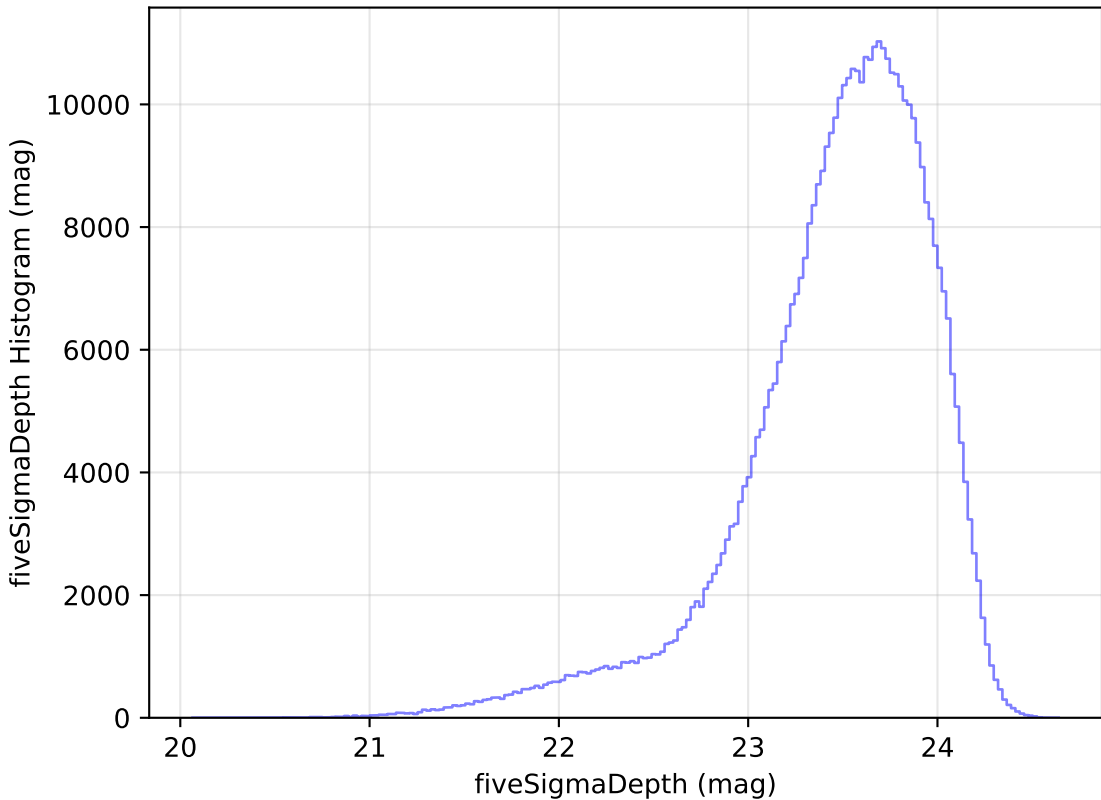
too_elab_r8_d3_gz_v3.4_10yrs i: fiveSigmaDepth Histogram
