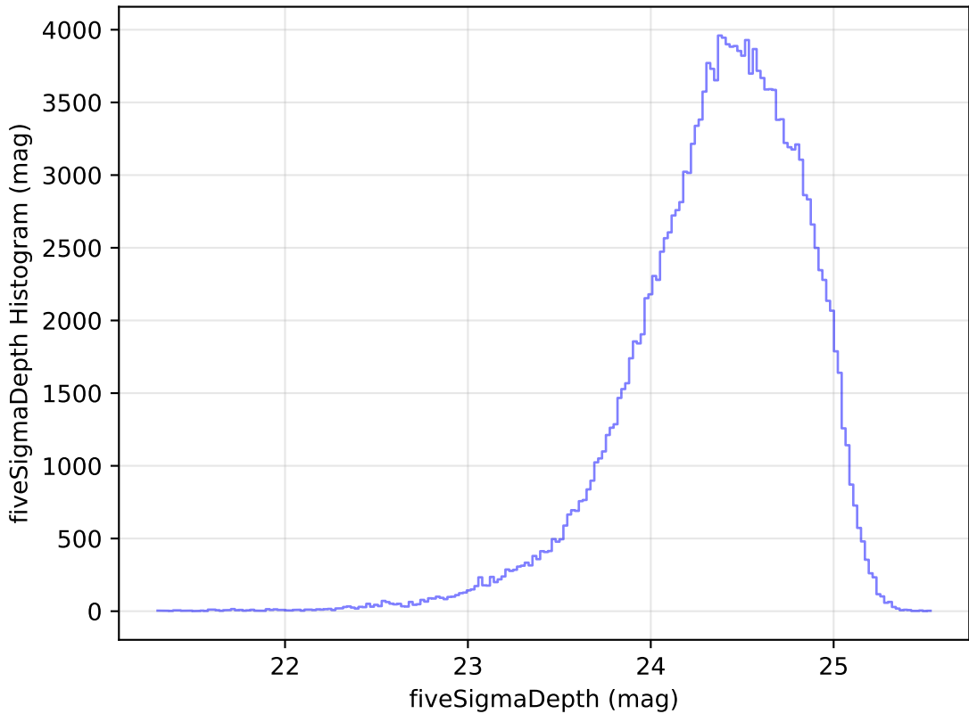
too_elab_r8_d3_gz_v3.4_10yrs g: fiveSigmaDepth Histogram
