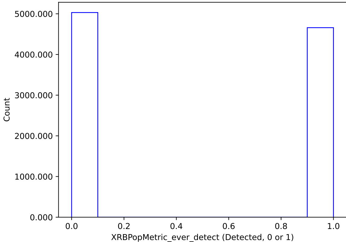
too_elab_r8_d3_gz_v3.4_10yrs : XRBPoMetric_ever_detect
