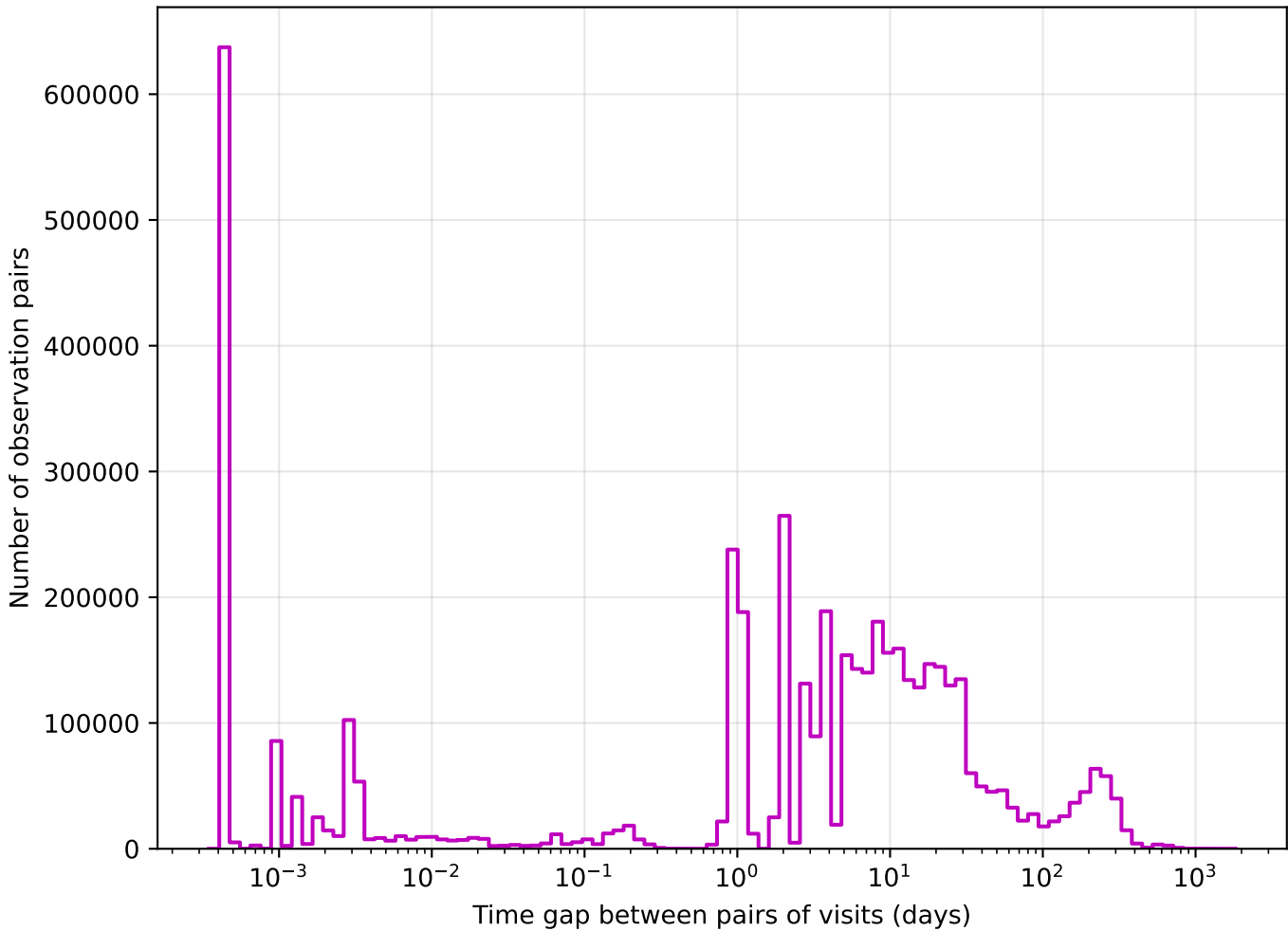
too_elab_r8_d3_gz_v3.4_10yrs z band: Tgaps observationStartMJD
