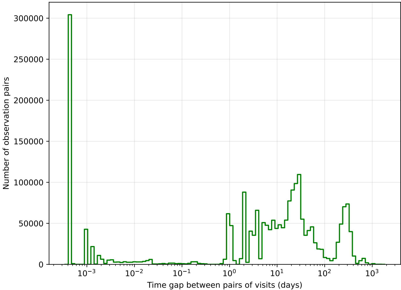
too_elab_r8_d3_gz_v3.4_10yrs g band: Tgaps observationStartMJD
