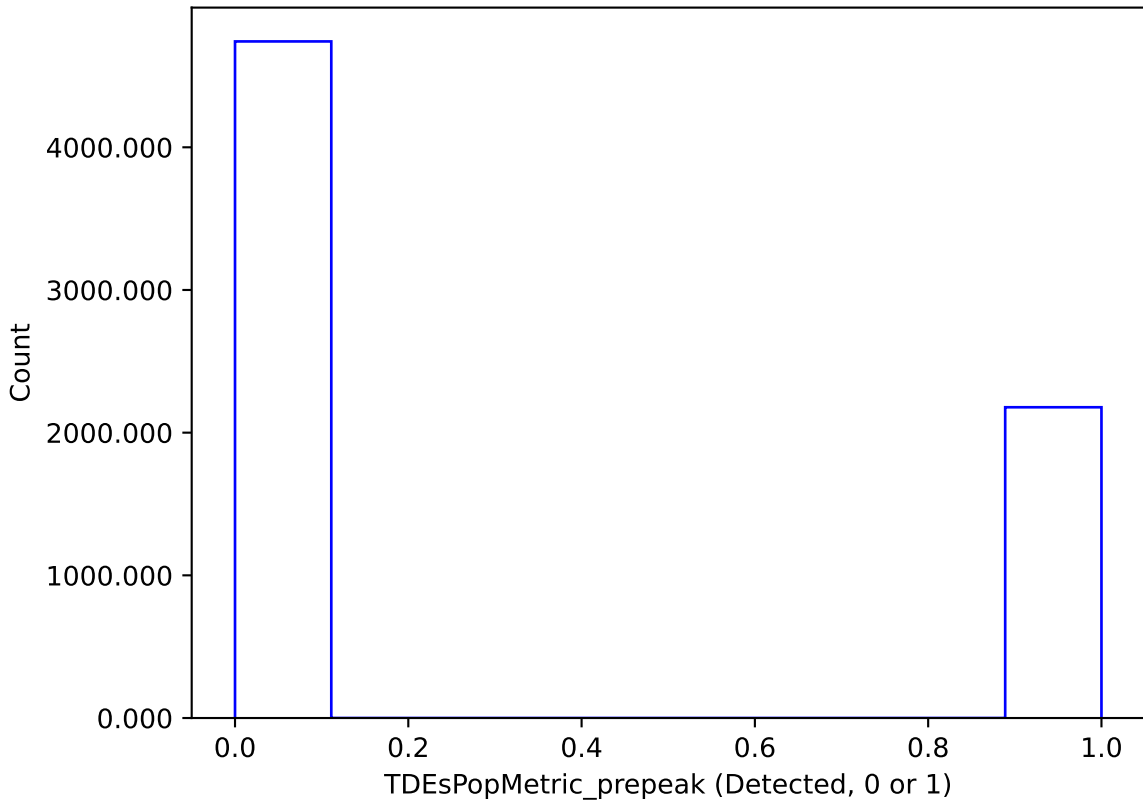
too_elab_r8_d3_gz_v3.4_10yrs : TDEsPopMetric_prepeak
