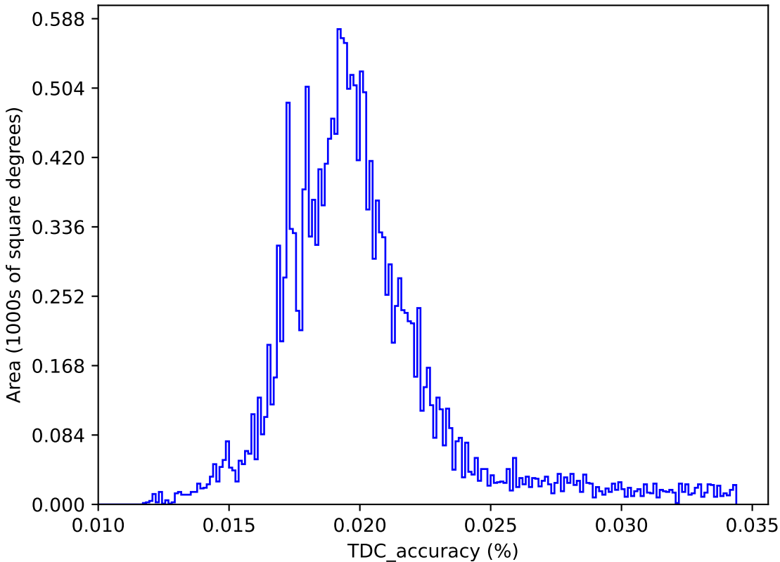
too_elab_r8_d3_gz_v3.4_10yrs : TDC_accuracy
