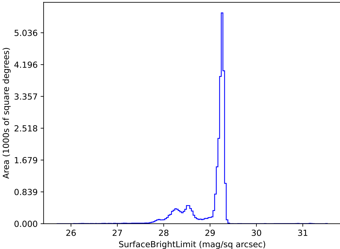
too_elab_r8_d3_gz_v3.4_10yrs z: SurfaceBrightLimit
