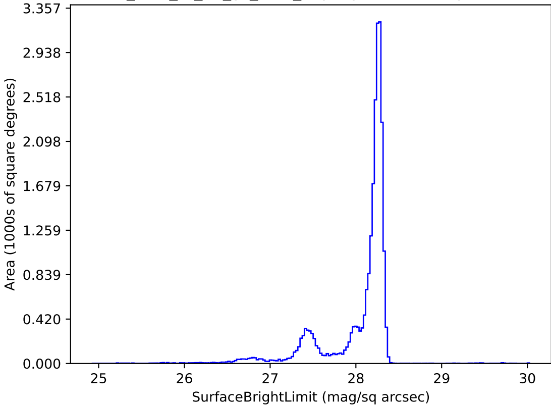
too_elab_r8_d3_gz_v3.4_10yrs y: SurfaceBrightLimit
