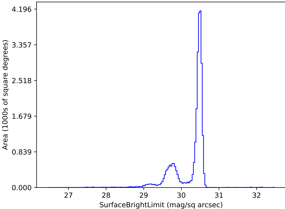
too_elab_r8_d3_gz_v3.4_10yrs r: SurfaceBrightLimit
