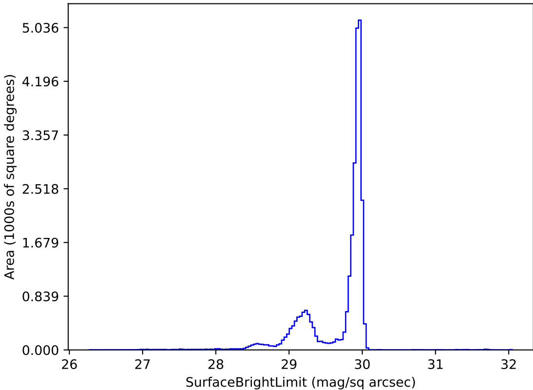
too_elab_r8_d3_gz_v3.4_10yrs i: SurfaceBrightLimit
