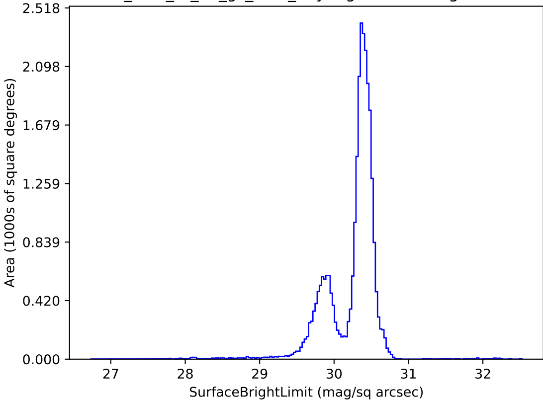
too_elab_r8_d3_gz_v3.4_10yrs g: SurfaceBrightLimit
