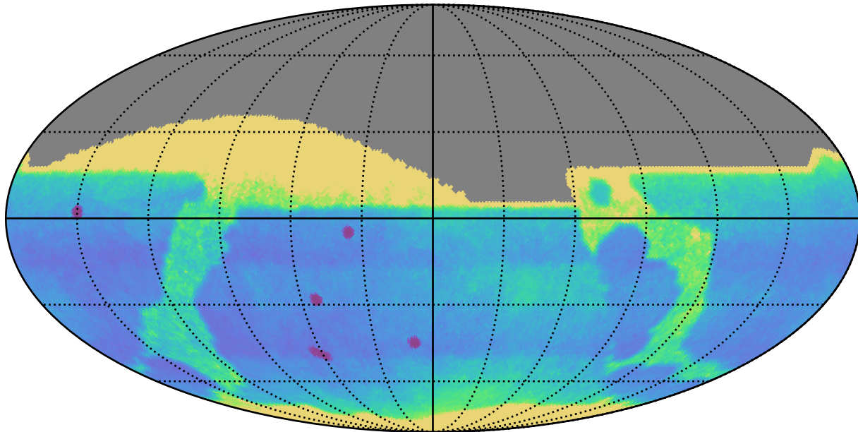
too_elab_r8_d3_gz_v3.4_10yrs : Proper Motion Uncert @ 24.0
