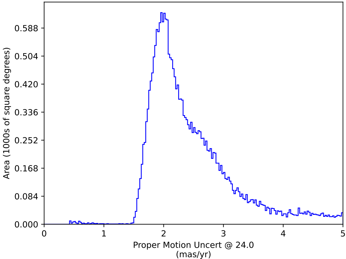
too_elab_r8_d3_gz_v3.4_10yrs : Proper Motion Uncert @ 24.0
