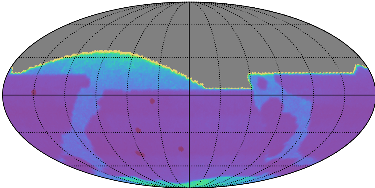
too_elab_r8_d3_gz_v3.4_10yrs : Proper Motion Uncert @ 20.5
