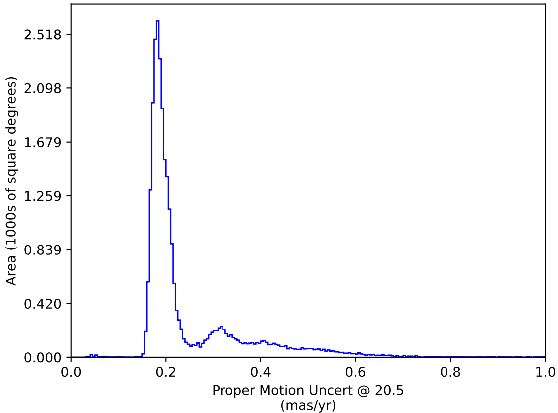
too_elab_r8_d3_gz_v3.4_10yrs : Proper Motion Uncert @ 20.5
