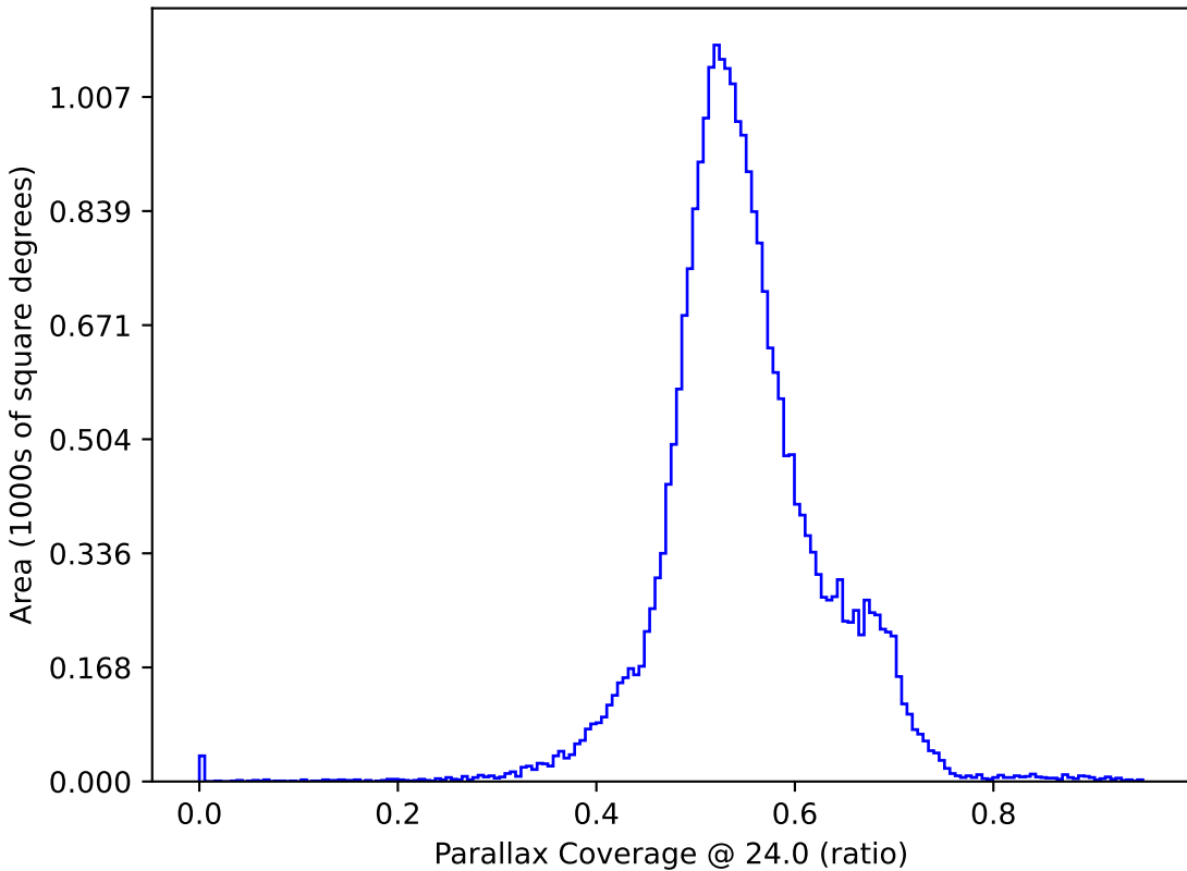
too_elab_r8_d3_gz_v3.4_10yrs : Parallax Coverage @ 24.0
