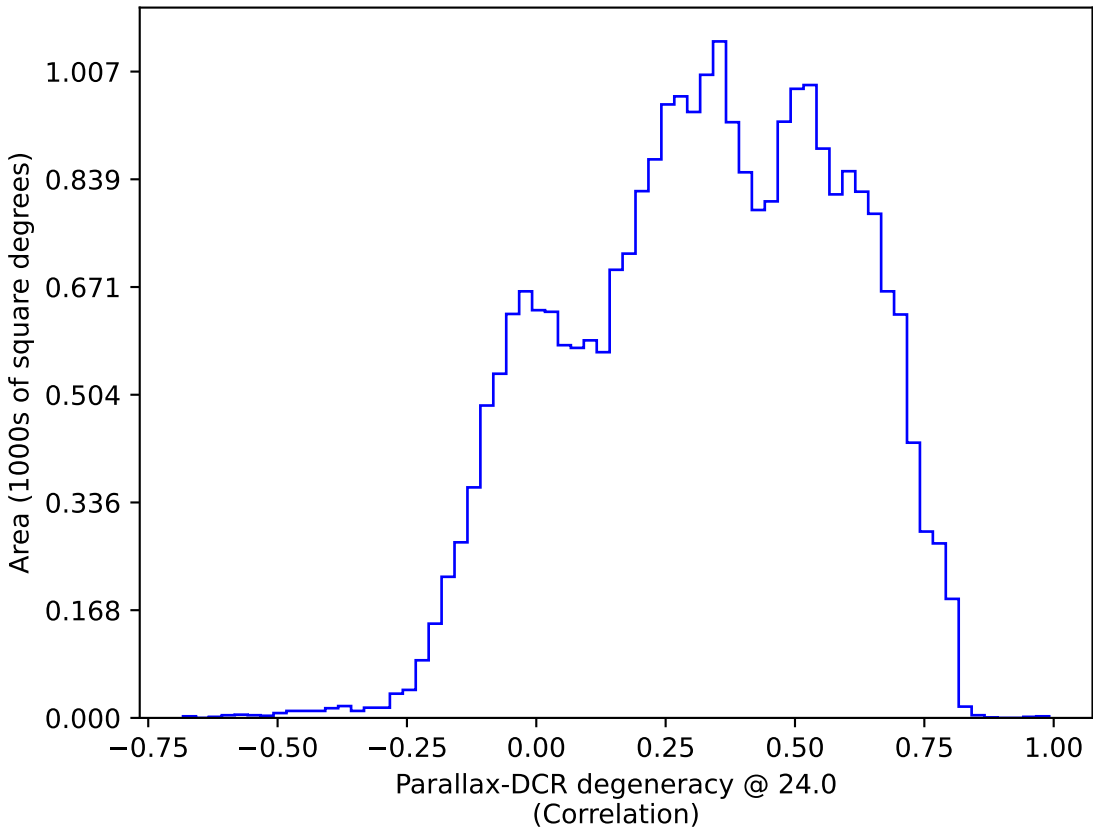
too_elab_r8_d3_gz_v3.4_10yrs : Parallax-DCR degeneracy @ 24.0
