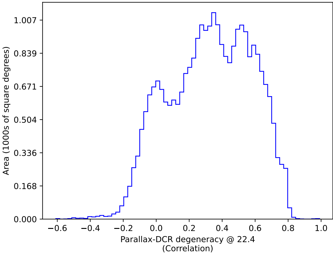
too_elab_r8_d3_gz_v3.4_10yrs : Parallax-DCR degeneracy @ 22.4
