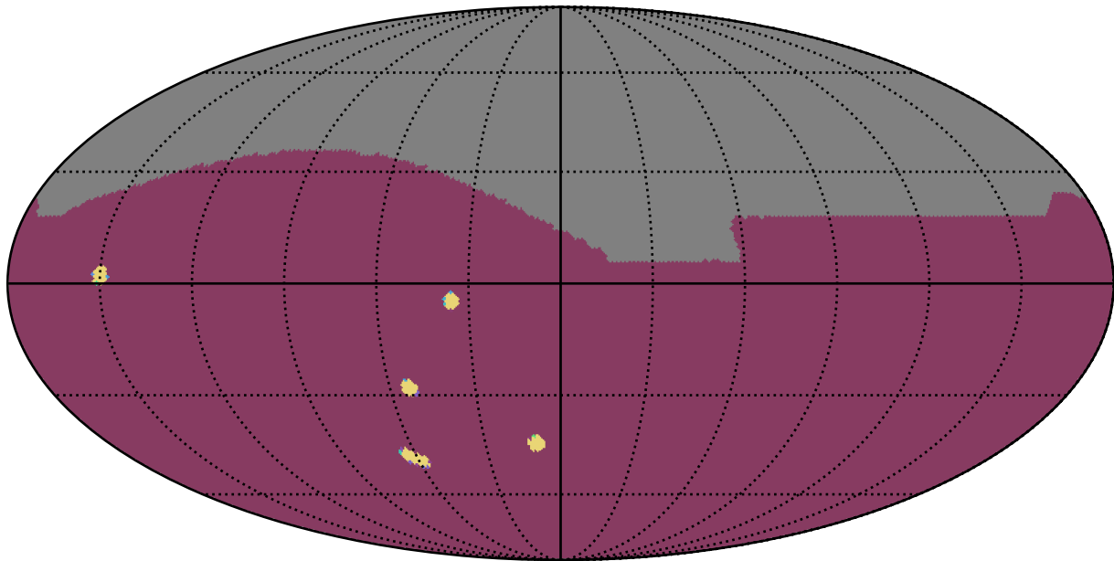
too_elab_r8_d3_gz_v3.4_10yrs : NumberOfQuickRevisits
