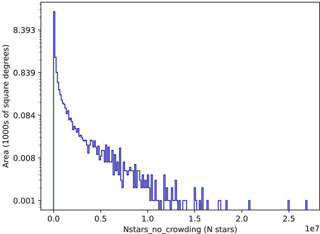
too_elab_r8_d3_gz_v3.4_10yrs i: Nstars_no_crowding
