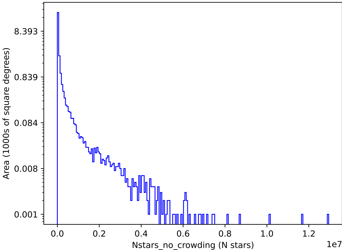
too_elab_r8_d3_gz_v3.4_10yrs g: Nstars_no_crowding
