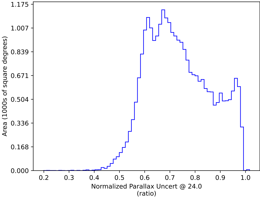
too_elab_r8_d3_gz_v3.4_10yrs : Normalized Parallax Uncert @ 24.0
