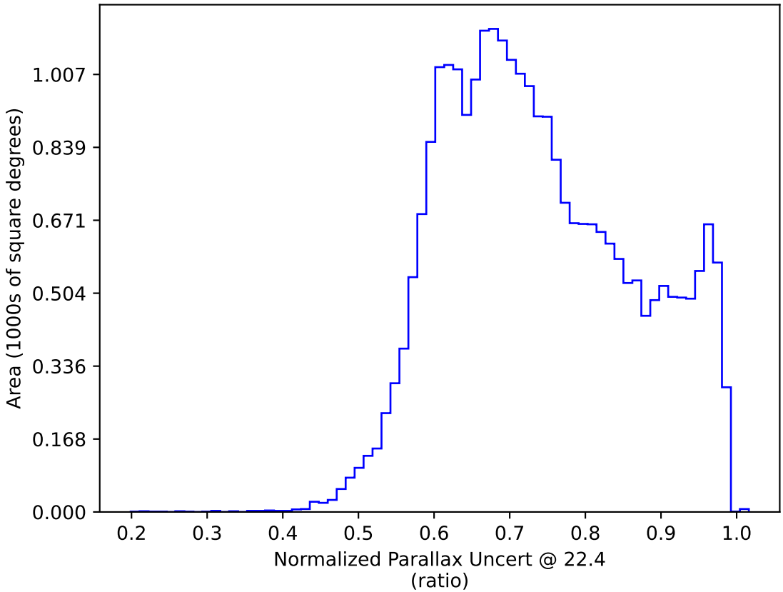
too_elab_r8_d3_gz_v3.4_10yrs : Normalized Parallax Uncert @ 22.4
