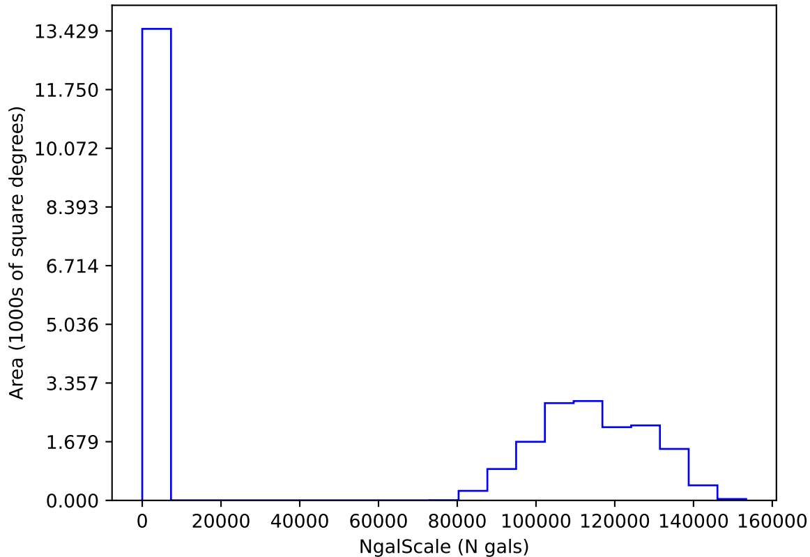
too_elab_r8_d3_gz_v3.4_10yrs i: NgalScale
