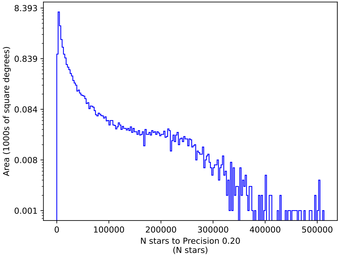
too_elab_r8_d3_gz_v3.4_10yrs u: N stars to Precision 0.20
