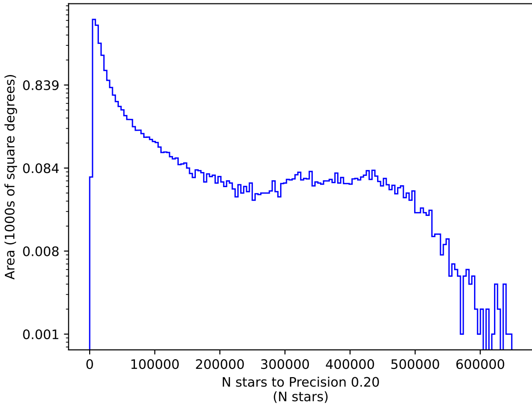
too_elab_r8_d3_gz_v3.4_10yrs r: N stars to Precision 0.20
