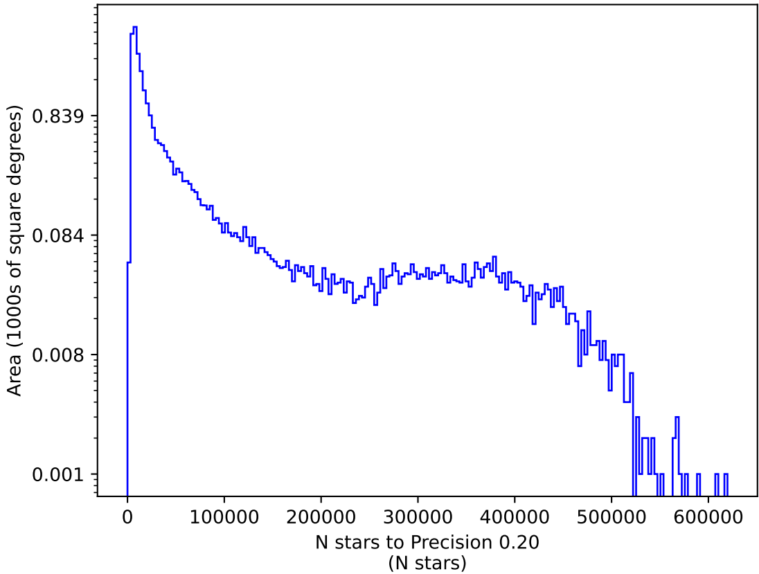
too_elab_r8_d3_gz_v3.4_10yrs g: N stars to Precision 0.20
