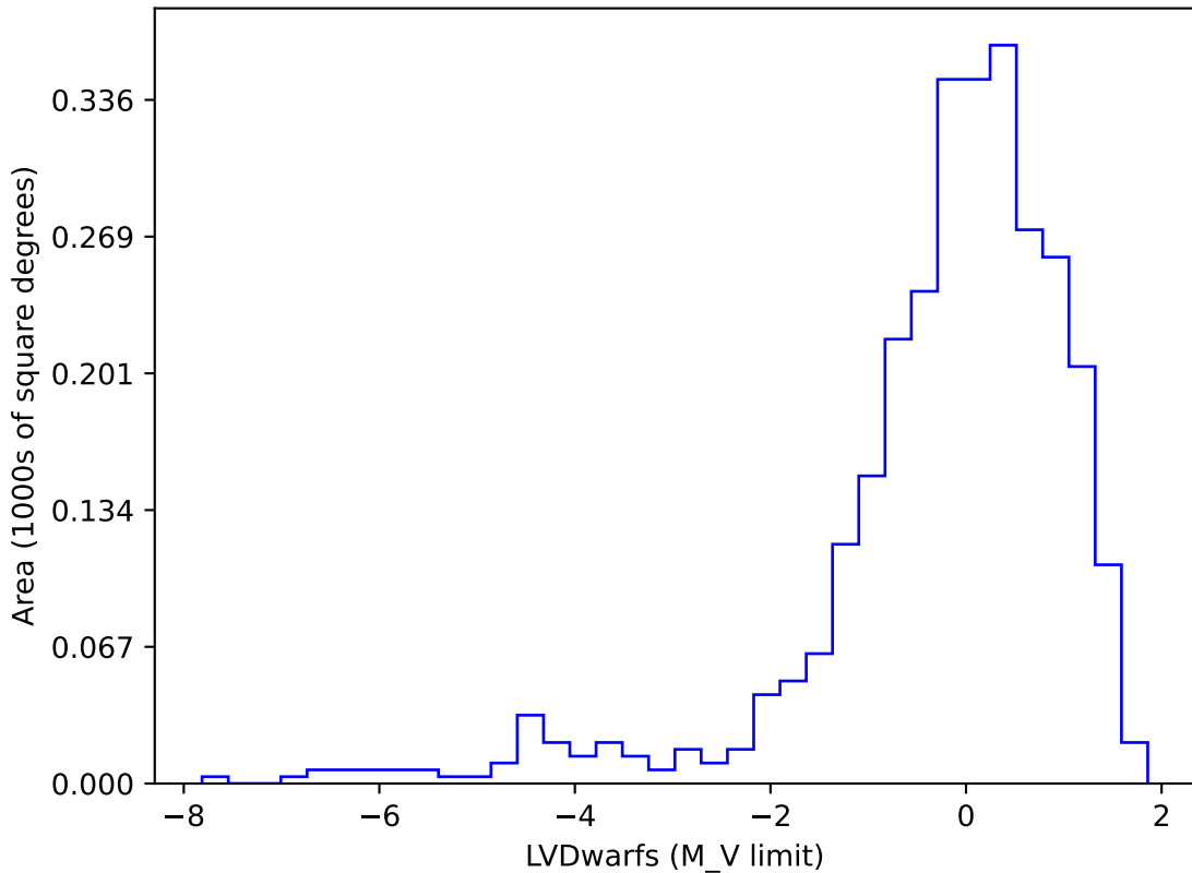
too_elab_r8_d3_gz_v3.4_10yrs gi SCP: LVDwarfs
