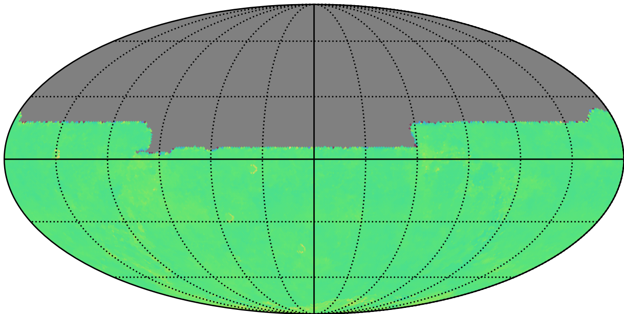
too_elab_r8_d3_gz_v3.4_10yrs y: Kuiper rotTelPos
