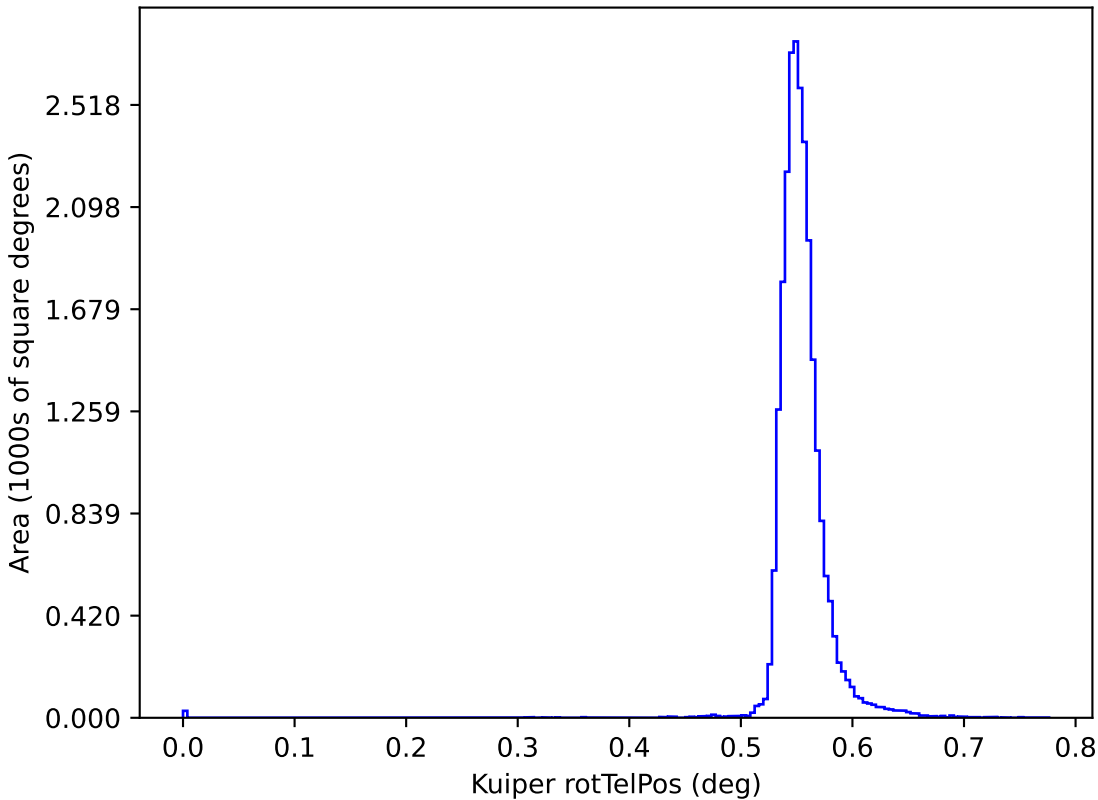
too_elab_r8_d3_gz_v3.4_10yrs y: Kuiper rotTelPos
