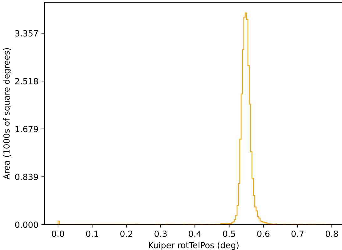
too_elab_r8_d3_gz_v3.4_10yrs r: Kuiper rotTelPos
