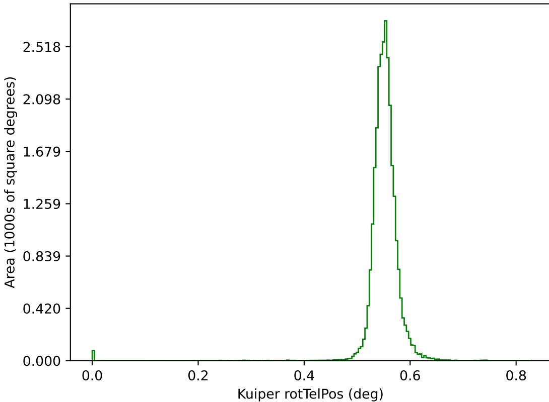
too_elab_r8_d3_gz_v3.4_10yrs g: Kuiper rotTelPos
