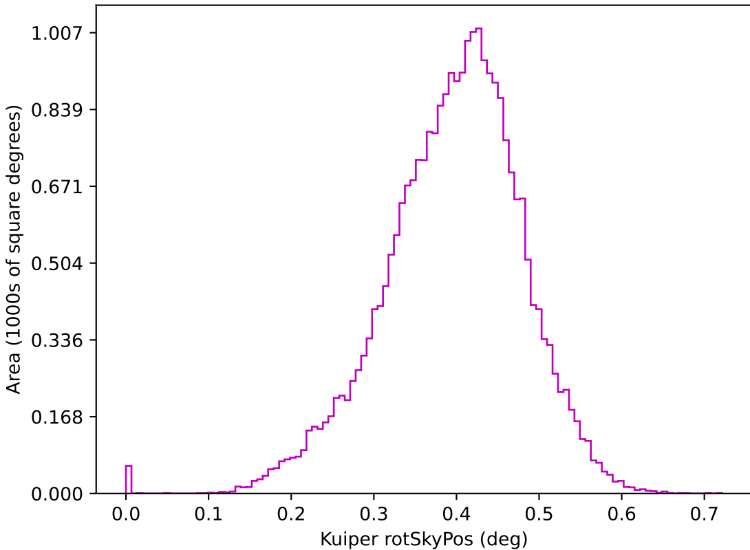
too_elab_r8_d3_gz_v3.4_10yrs z: Kuiper rotSkyPos
