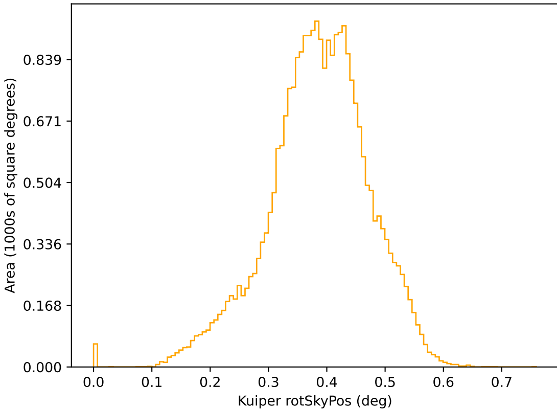
too_elab_r8_d3_gz_v3.4_10yrs r: Kuiper rotSkyPos
