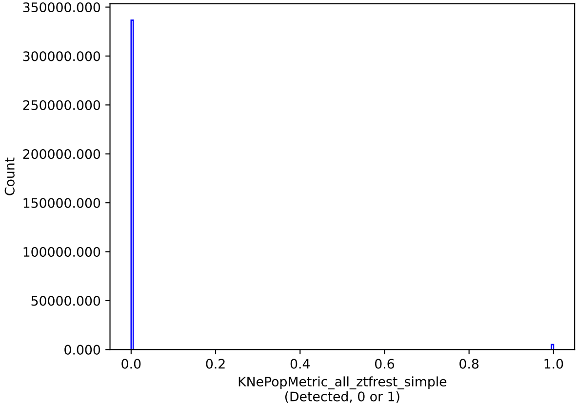
too_elab_r8_d3_gz_v3.4_10yrs all models: KNePopMetric_all_ztfrest_simple
