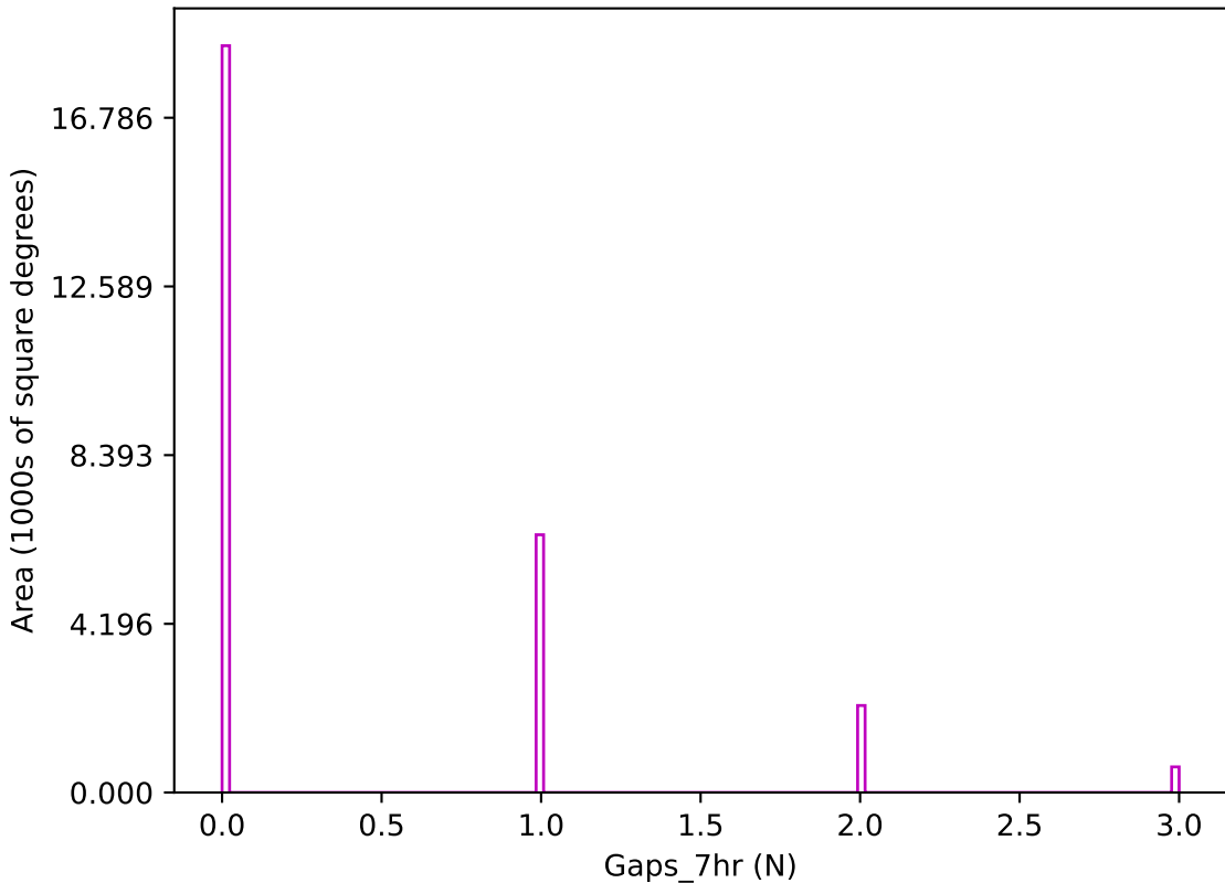
too_elab_r8_d3_gz_v3.4_10yrs z band: Gaps_7hr
