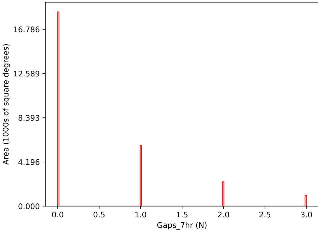
too_elab_r8_d3_gz_v3.4_10yrs i band: Gaps_7hr
