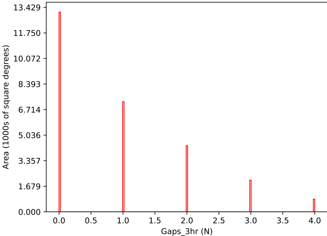
too_elab_r8_d3_gz_v3.4_10yrs i band: Gaps_3hr
