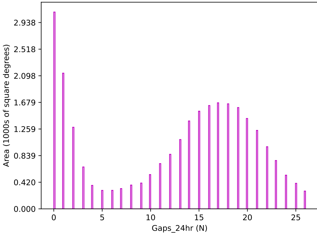
too_elab_r8_d3_gz_v3.4_10yrs z band: Gaps_24hr
