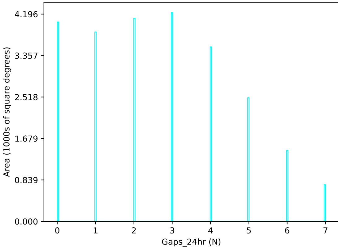
too_elab_r8_d3_gz_v3.4_10yrs u band: Gaps_24hr
