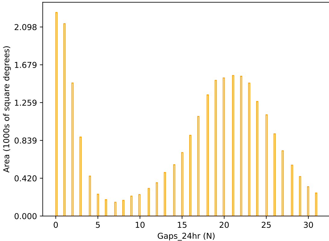
too_elab_r8_d3_gz_v3.4_10yrs r band: Gaps_24hr
