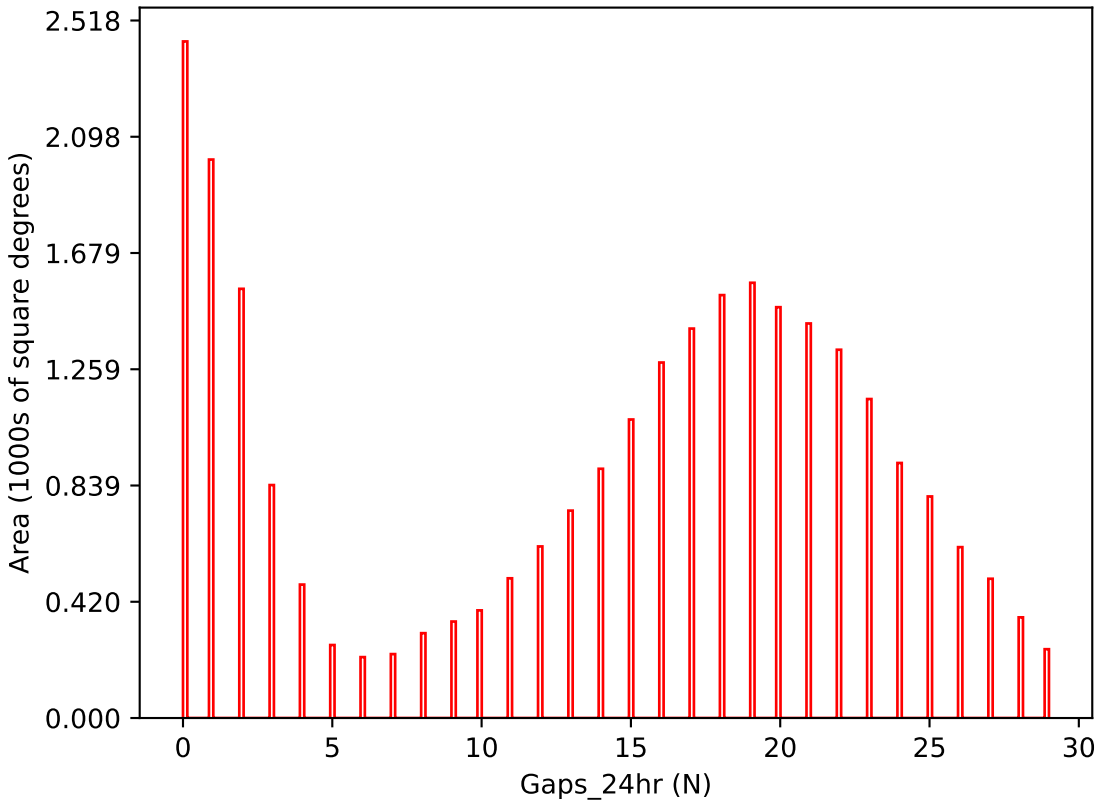
too_elab_r8_d3_gz_v3.4_10yrs i band: Gaps_24hr
