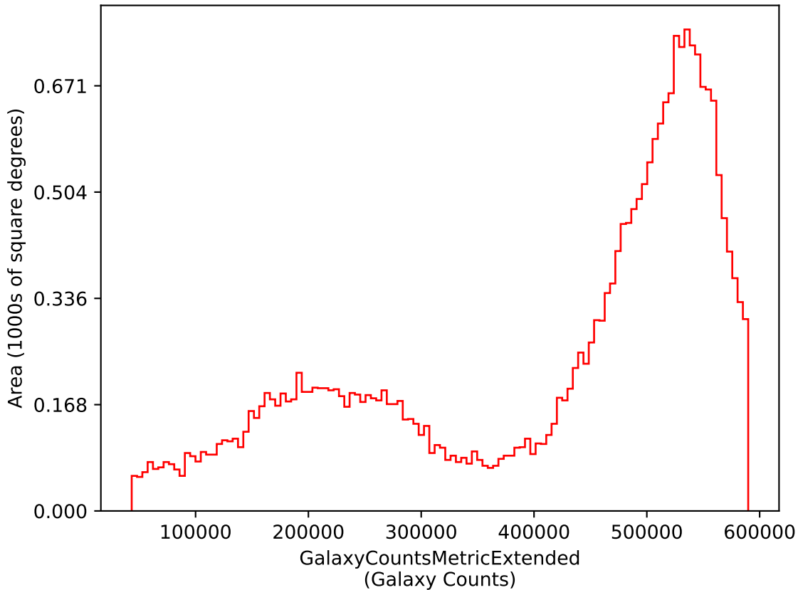
too_elab_r8_d3_gz_v3.4_10yrs i: GalaxyCountsMetricExtended
