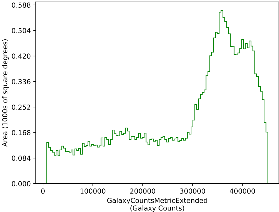
too_elab_r8_d3_gz_v3.4_10yrs g: GalaxyCountsMetricExtended
